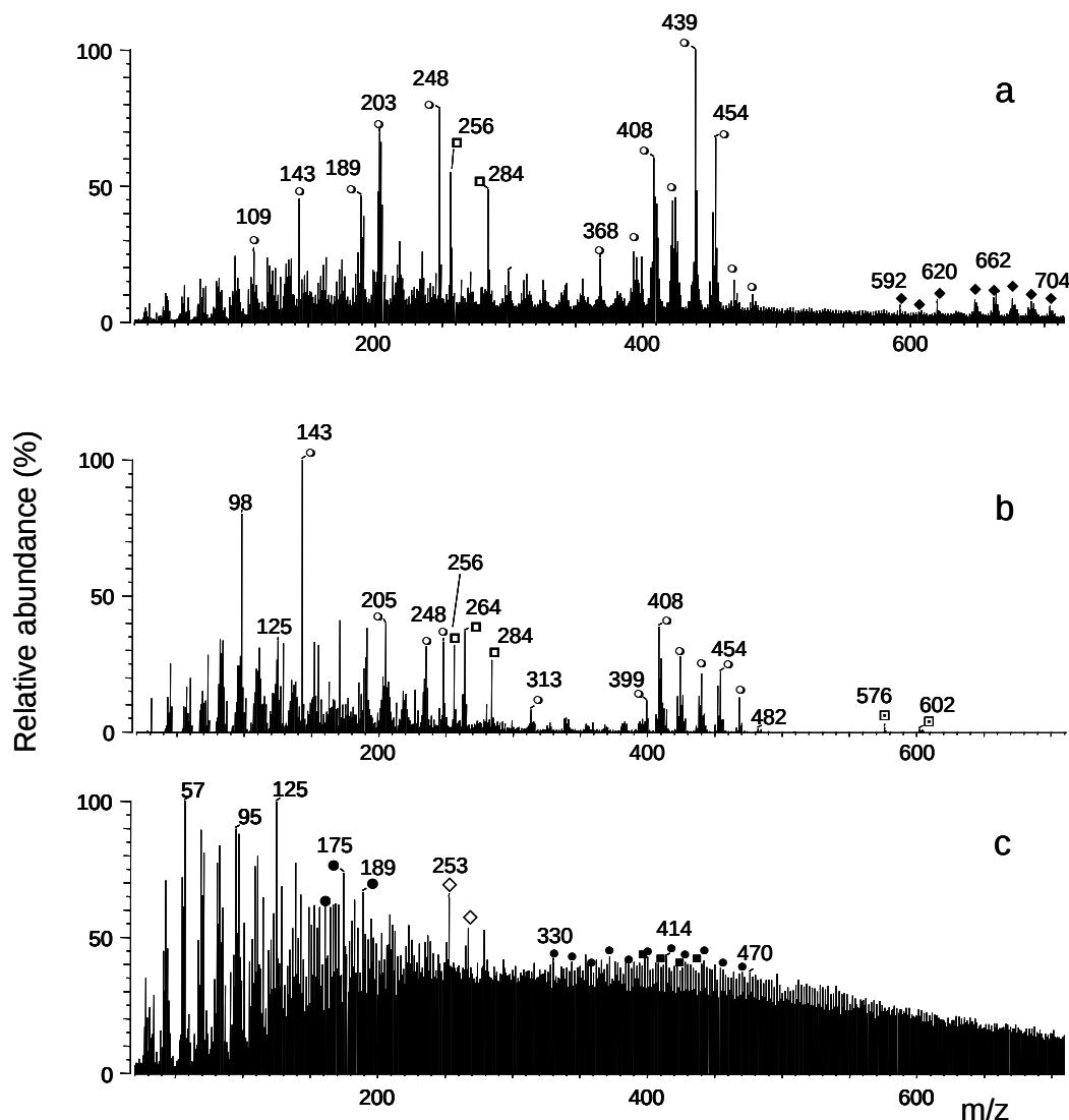
Fig. 1. DTMS summation spectra of: (a) Hafkenschid mummy pigment sample (MP), (b) Hafkenschid asphalt sample (A) and (c) megilp sample (MG).
