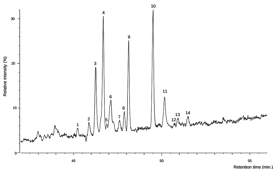
Fig. 6. On-column GC/MS retention window of the methylated triterpenoid compounds from mastic in the Hafkenschied mummy pigment sample (MP).
