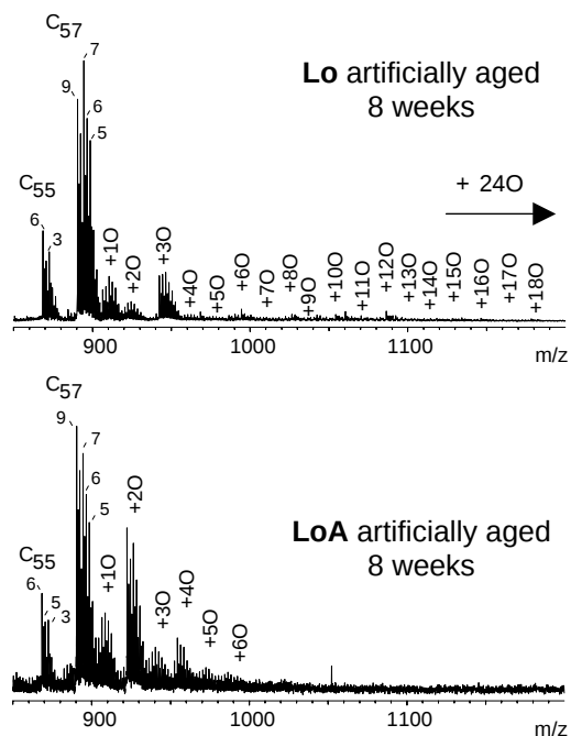
Fig. 1. Partial ESI-FTMS showing autooxidation (i.e. photo-oxidation) of linseed oil artificially aged for 8 weeks as such (incorporation of up to 24 atoms of O) and in the presence of asphalt (only 6 fold oxygenation).
