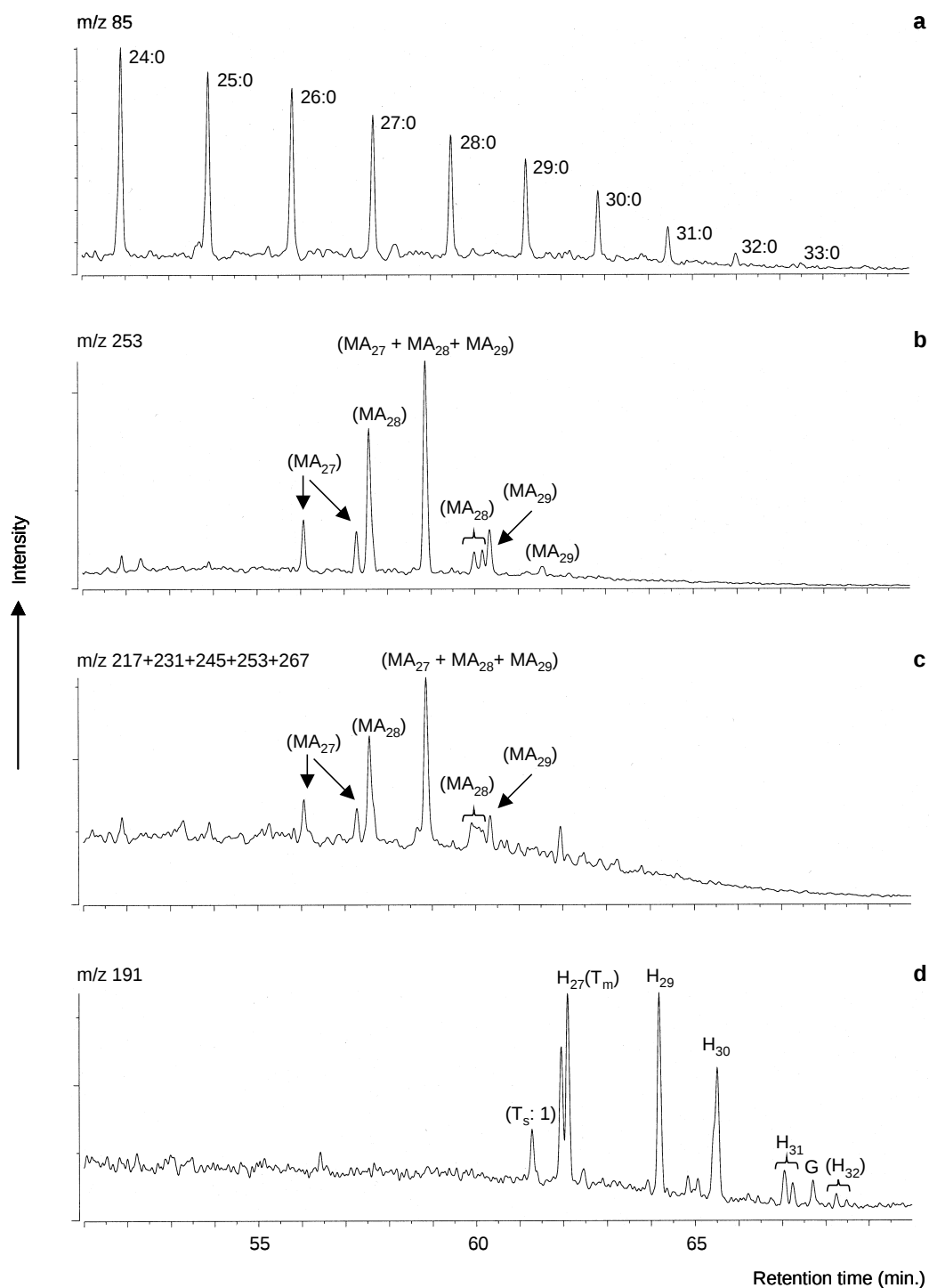
Fig. 5. Partial mass chromatograms of (a) alkanes as markers for aliphatic cross-links (m/z 85), (b) C-ring monoaromatic steroids MA_i (m/z 253), (c) steroid hydrocarbons (m/z 217+231+245+253+267) and biomarker (d) hopanes H_i (m/z 191) in Py-GC/MS data of sample HS.
