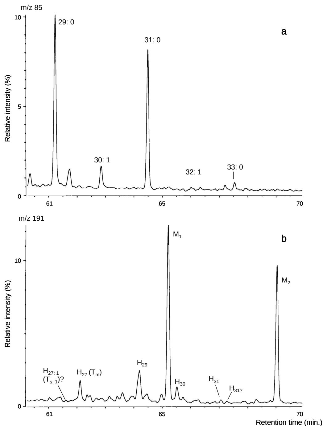
Fig. 2. Py-GC/MS partial mass chromatogram of (a) alkanes as markers for aliphatic cross-links ( m/z 85) and (b) hopanoid compounds, H_i ( m/z 191) in the Hafkenschied mummy pigment sample (MP); M_1 and M_2 are isotopic contributions of mastic resin components to m/z 191.
