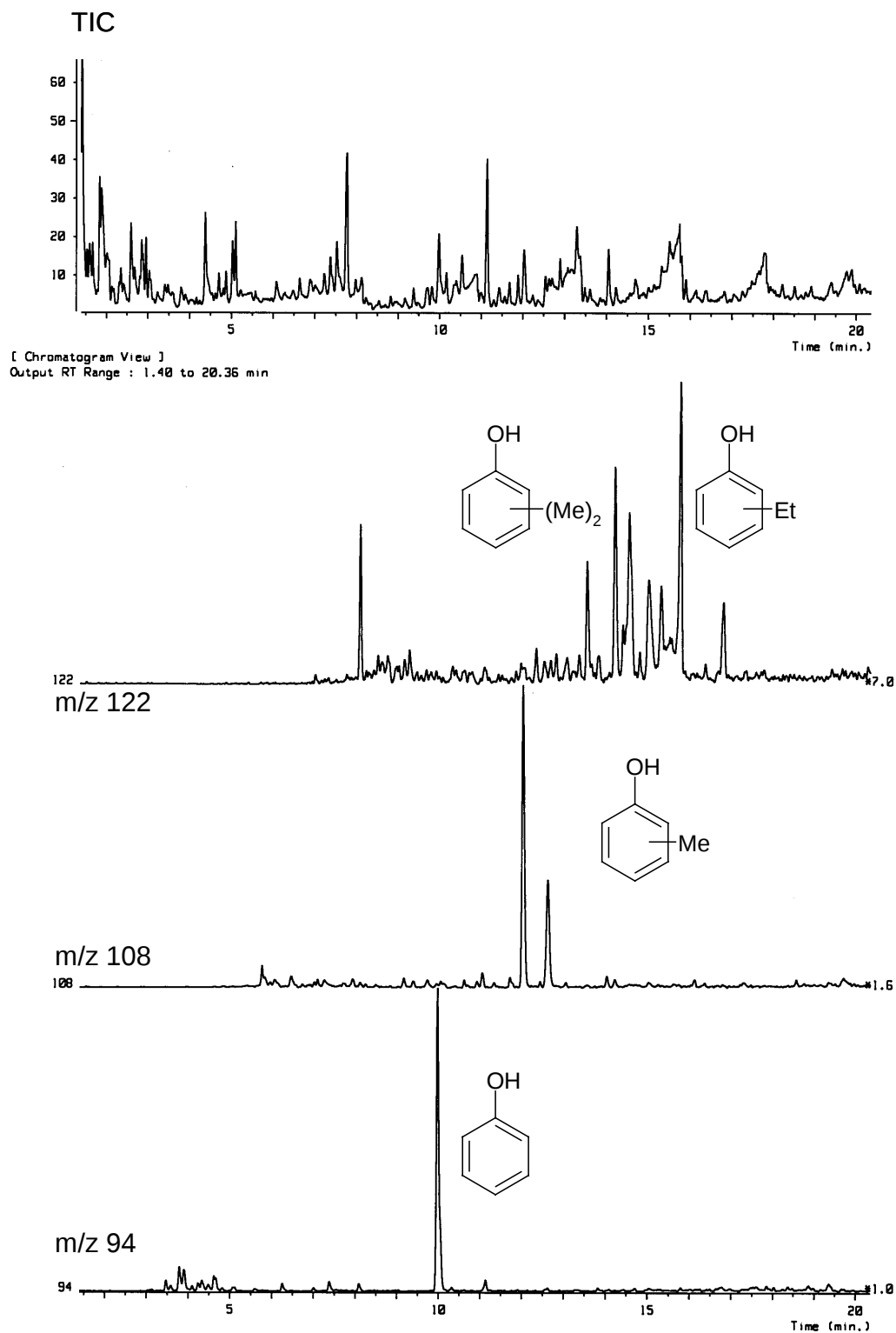
Fig. 18. Phenolic compounds in an oil paint sample (Re 1 ) suspected of asphalt addition from 'Death of Dido' by Sir Joshua Reynolds.
