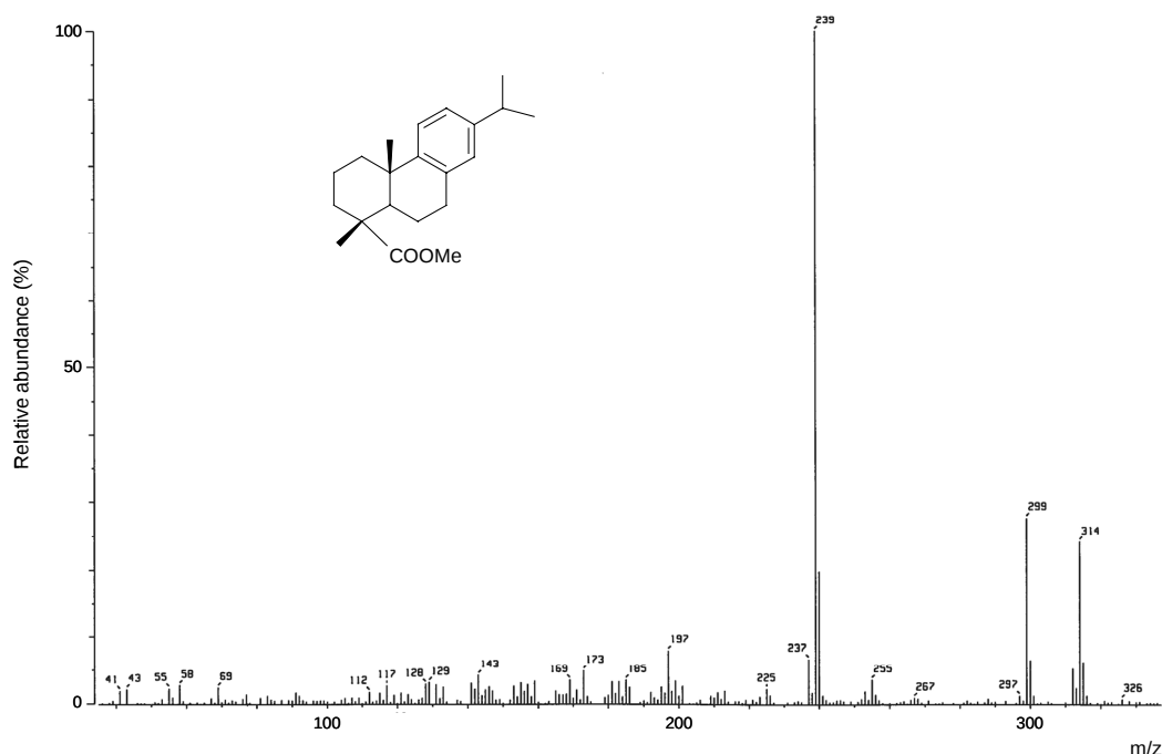
Fig. 5. Mass spectrum and formula of dehydroabietic acid (DHA) in Py-TMAH-GC/MS data of the Hafkenschied mummy pigment sample (MP).
