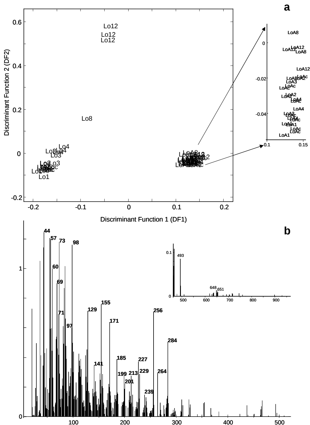
Fig. 10. Discriminant analytical map of the chemical composition (DTMS data) of VEGA asphalt-linseed oil DCM test solutions (right) in comparison with linseed oil DCM test solutions comparing initial state (control) and solutions artificially aged for 1, 2, 3, 4, 8 and 12 weeks (a). Mass spectrum of the DF2 (b).
