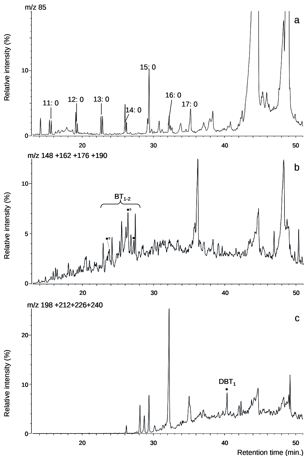
Fig. 3. Py-GC/MS partial mass chromatogram of (a) alkanes as markers for aliphatic cross-links (m/z 85) (b) alkyl-benzothiophenes (m/z 148+ 162+ 176+ 190) and (c) alkyl-dibenzothiophenes (m/z 198+ 212+ 226+ 240) in the Hafkenschied mummy pigment sample (MP).
