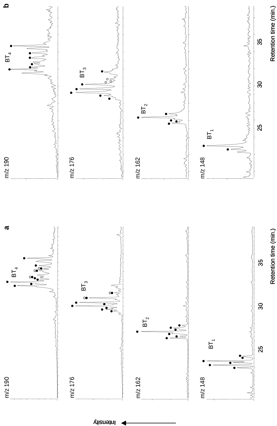
Fig. 9. Partial mass chromatograms of alkylbenzothiophenes BT_i of sample HS (a) and sample DS (b) in Py-GC/MS data; '•' is used to mark the saturated compounds and 'o' the unsaturated homologues.
